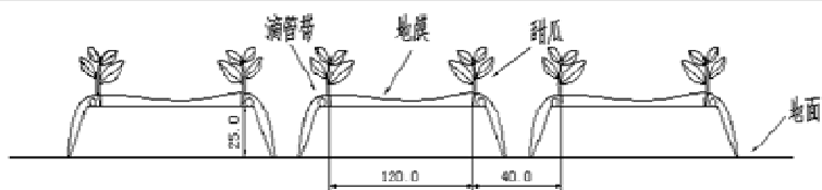
(a) CK小区甜瓜种植方式和滴灌带、地膜布置
